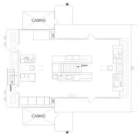
DECK 03
