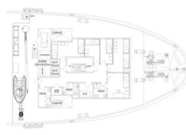
DECK 01
