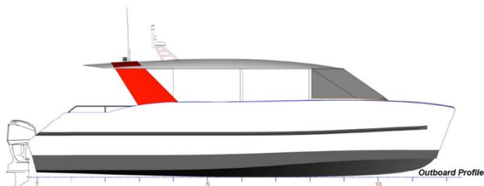
SFM 12m Dive Catamaran
