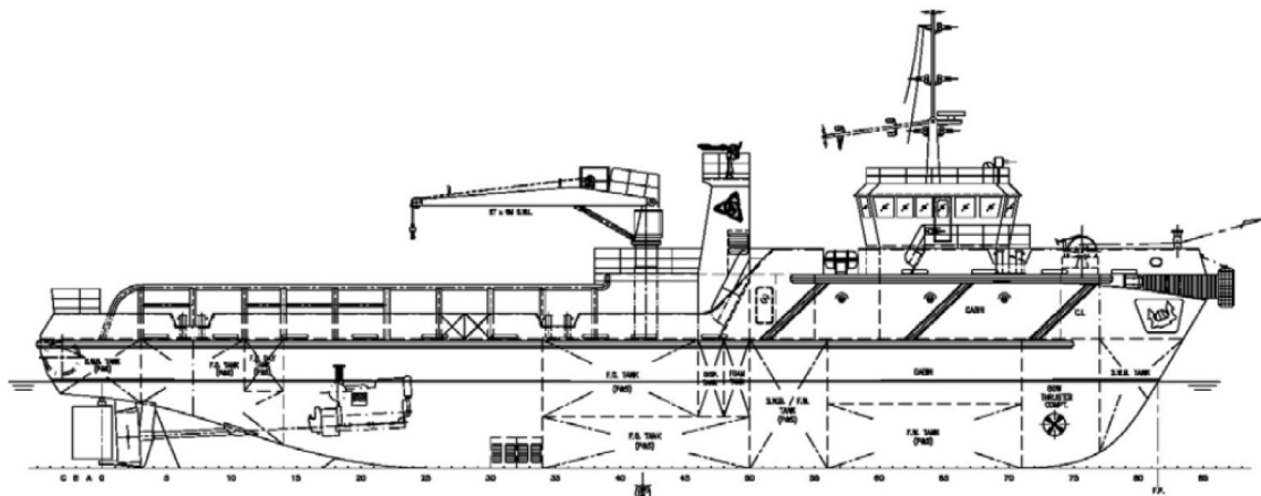
OUTBOARD PROFILE
