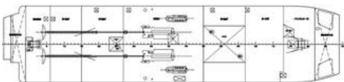
LOWER DECK
