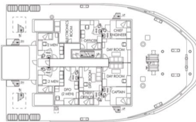
UPPER FORECASTLE DECK
