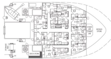
FORECASTLE DECK
