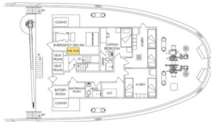
DECK 01
