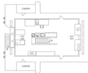
DECK 02
