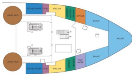
LOWER DECK
