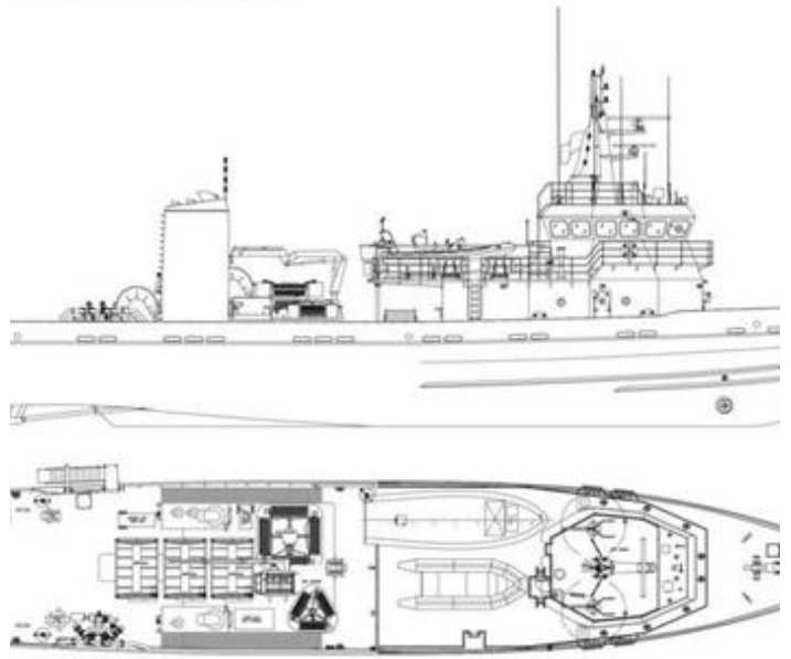
MULTI PURPOSE VESSEL
