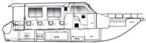
③ MIDSHIP SECTION (PS)
