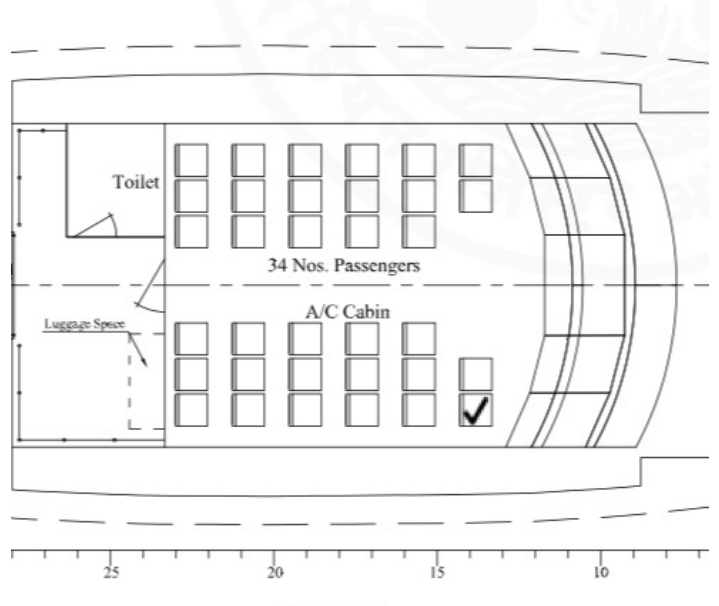
UPPER DECK
