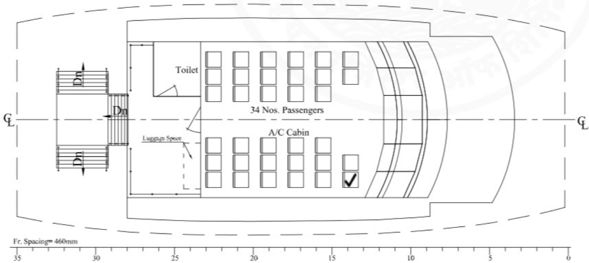
UPPER DECK
