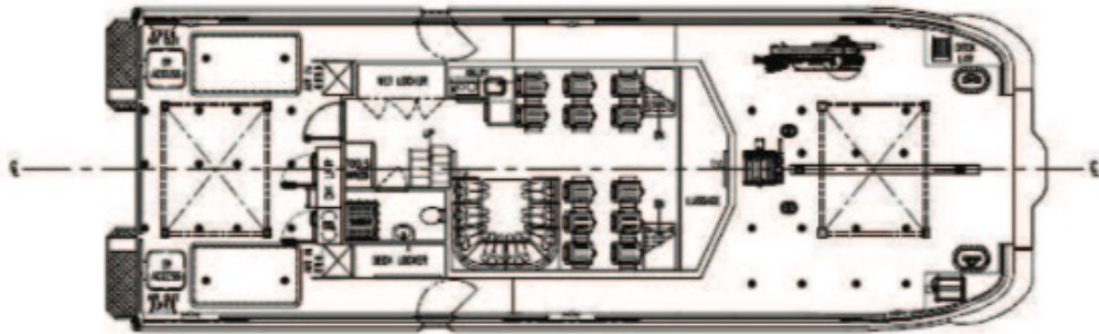
PLAN VIEW ON MAIN DECK
