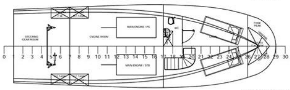
BELOW MAINDECK
